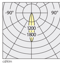
35 W/3500 lm Efficiency 62% α=22°
