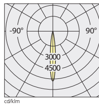
70 W/6900 lm Efficiency 54% α=12°
