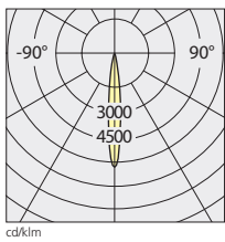
35 W/3500 lm Efficiency 54% α=12°
