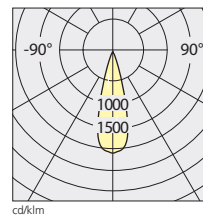
35 W/3500 lm Efficiency 59% α=28°
