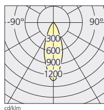
70 W/6900 lm Efficiency 63% α=38°
