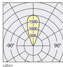
27 W 3000 K α=38°
