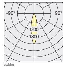
70 W/6900 lm Efficiency 62% α=22°
