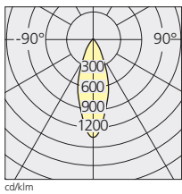
35 W/3500 lm Efficiency 63% α=38°
