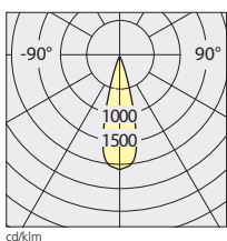
70 W/6900 lm Efficiency 59% α=28°
