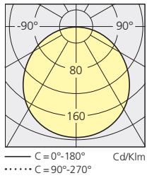
Prismatic glass diffuser
