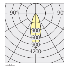
70 W/6200 lm
